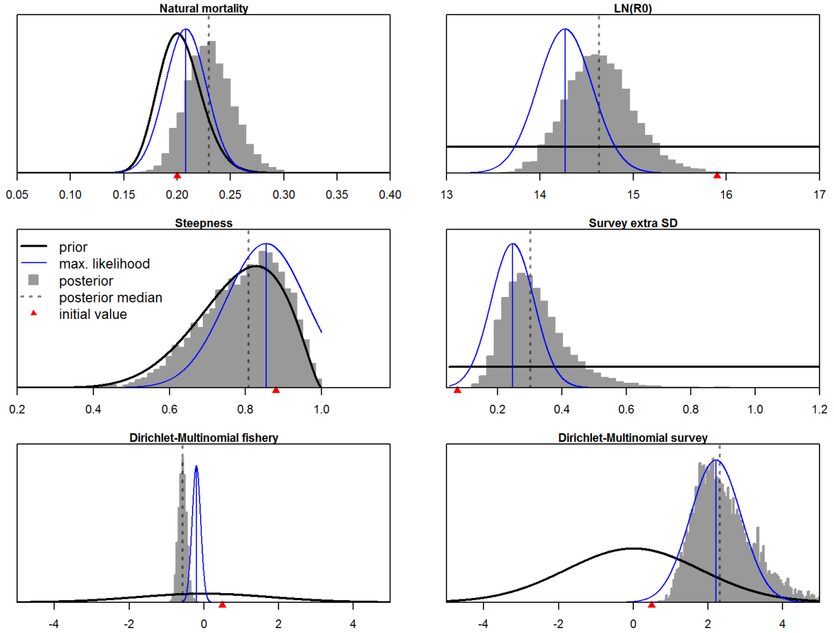
Figure 20. Prior (black lines) and posterior (gray histograms) distributions for key parameters in the base model. The parameters are: natural mortality ( M ), equilibrium log recruitment ( \log R_0 ), steepness ( h ), the additional process-error standard deviation for the acoustic survey, and the Dirichlet-Multinomial parameters for the fishery ( \theta_{\text{fish}} ) and the survey ( \theta_{\text{surv}} ). The maximum likelihood estimates and associated symmetric uncertainty intervals are also shown (blue lines). There are 50 bins for each posterior except the two Dirichlet-Multinomial parameters which are grouped into 500 bins.
