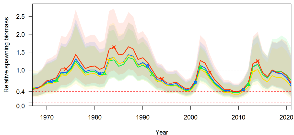
Figure 41. MCMC estimates of stock status (relative spawning biomass) for the base model and alternative sensitivity runs that represent changes in data. See Figure 40 for sensitivity descriptions.
