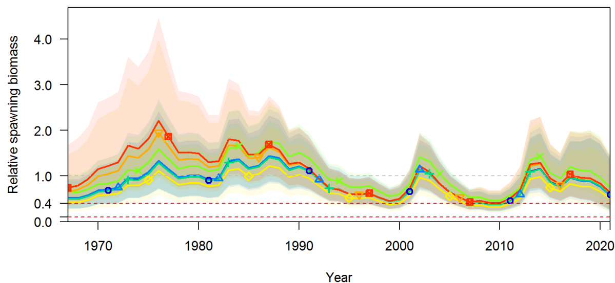
Figure 39. MCMC estimates of stock status (relative spawning biomass) for the base model and alternative sensitivity runs representing changing key parameters. See Figure 38 for sensitivity descriptions.
