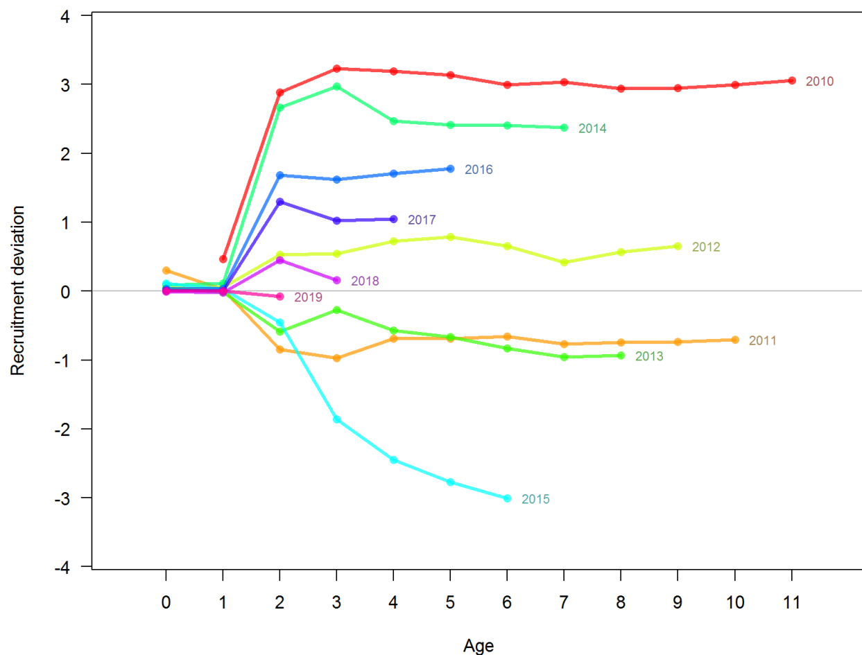
Figure G.1. Retrospective analysis of recruitment deviations from MCMC models over the last 6 years. Recruitment deviations are the log-scale differences between recruitment estimated by the model and expected recruitment from the spawner-recruit relationship. Lines represent estimated recruitment deviations for cohorts from 2010 to 2019, with cohort birth year marked at the right of each color-coded line. Values are estimated by models using data available only up to the year in which each cohort was a given age.
