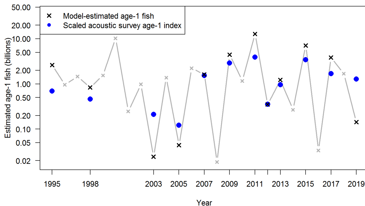
Figure 11. Preliminary acoustic survey age-1 index overlaid on estimated numbers of age-1 fish (medians of the posterior distribution from the base model).
