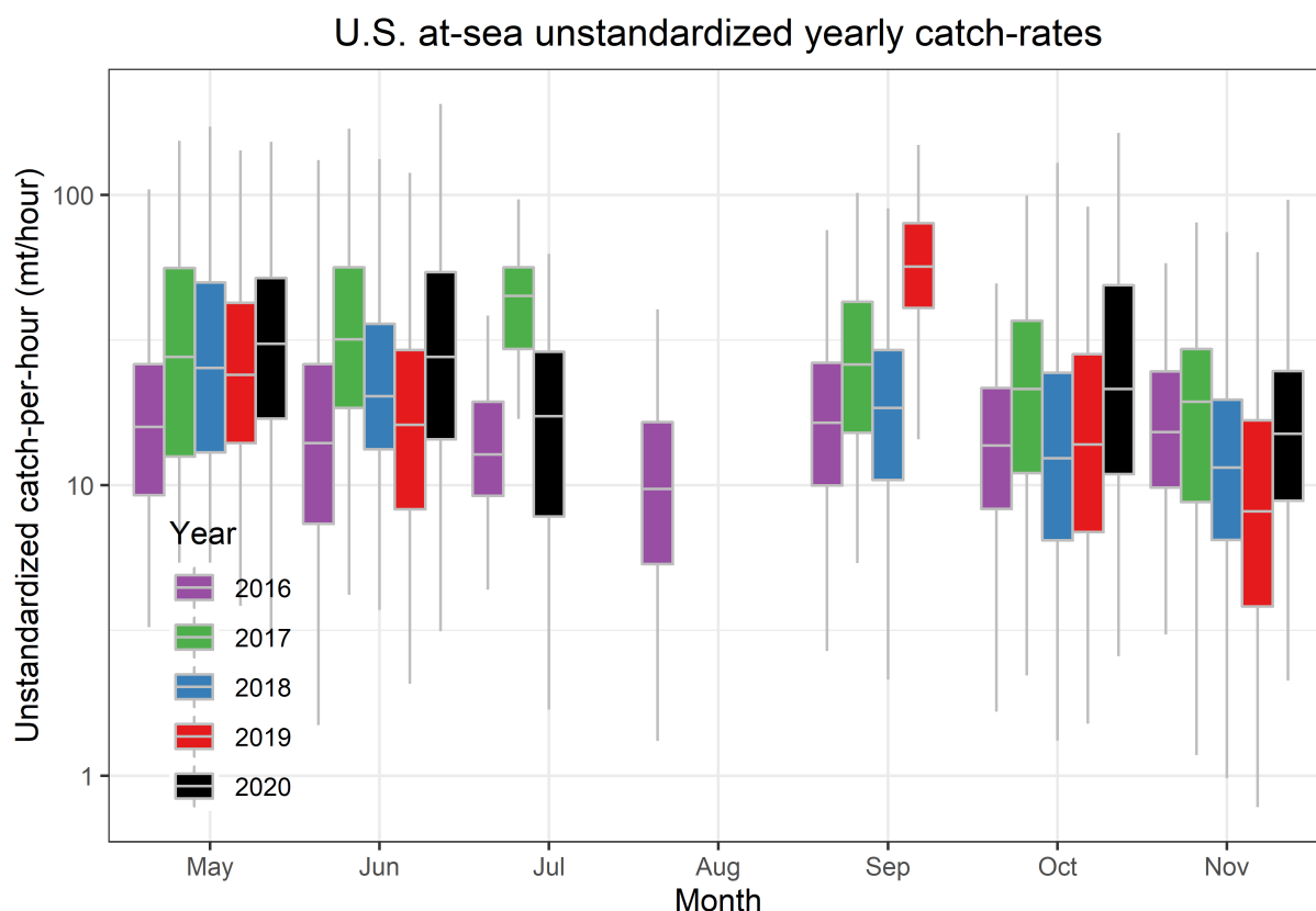
Figure 5. Unstandardized (raw) catch-rates (t/hr) of Pacific Hake catches by tow in the U.S. at-sea fleet from 2016–2020.
