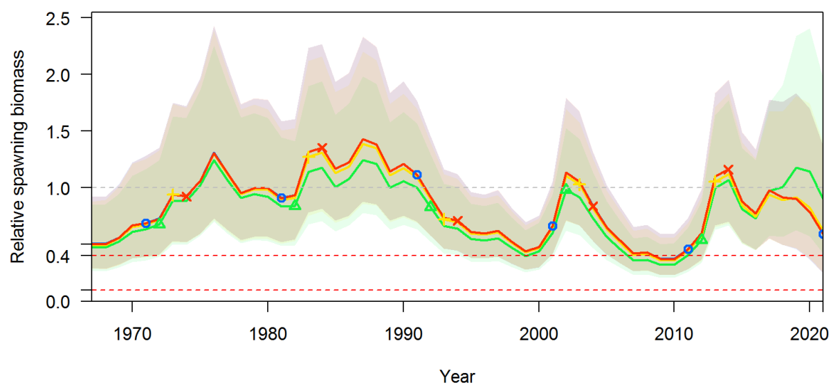
Figure 45. MCMC estimates of stock status (relative spawning biomass) for the base model and alternative sensitivity runs representing different standard deviations ( \Phi ) associated with time-varying selectivity. See Figure 44 for sensitivity descriptions.
