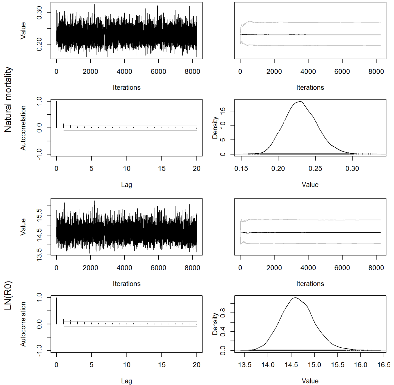
Figure A.1. Summary of MCMC diagnostics for natural mortality (upper panels) and the log of mean unfished equilibrium recruitment ( \ln(R_0) ; lower panels) in the base model. Top sub-panels show the trace of the sampled values across iterations (absolute values, top left; cumulative running mean with 5th and 95th percentiles, top right). The lower left sub-panel indicates the autocorrelation present in the chain at different lag times (i.e., distance between samples in the chain), and the lower right sub-panel shows the distribution of the values in the chain (i.e., the marginal density from a smoothed histogram of values in the trace plot).
