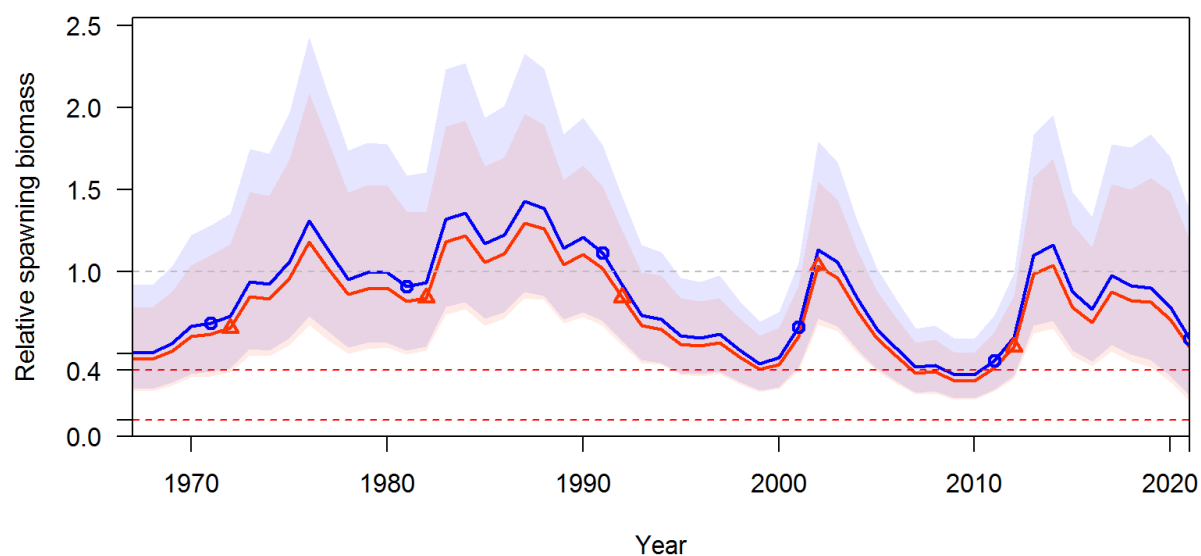
Figure H.2. MCMC median posterior estimates with 95% credible intervals of relative spawning biomass for the base model and alternative sensitivity run using rwMH.
