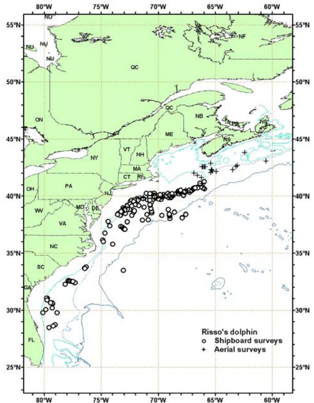
Figure 1. Distribution of Risso's dolphin sightings from NEFSC and SEFSC shipboard and aerial surveys during the summers of 1998, 1999, 2002, 2004 and 2006. Isobaths are the 100- m, 1,000- m, and 4,000-m depth contours.
