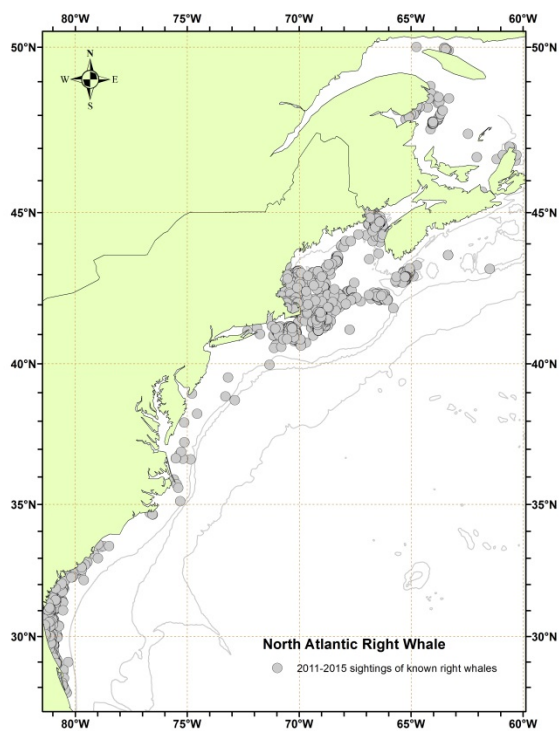
Figure 1. Distribution of sightings of known North Atlantic right whales, 2011-2015. Isobaths are the 100-m, 1000-m and 4000-m depth contours.
