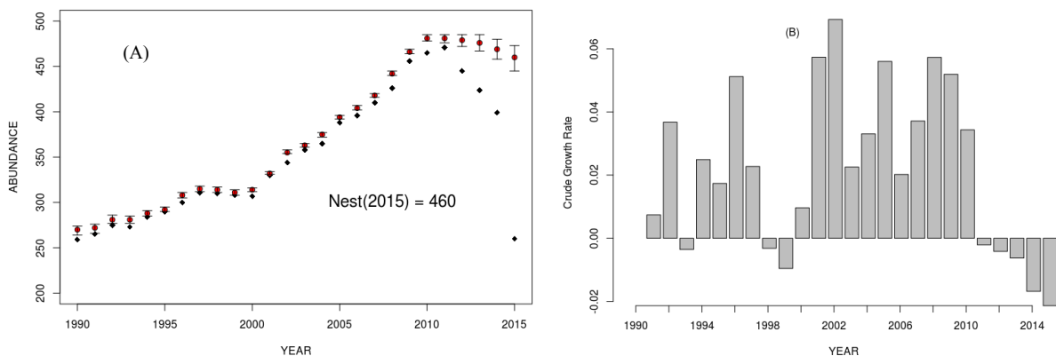
Figure 2. (A) Abundance estimates for North Atlantic right whales. Estimates are the median values of a posterior distribution from modeled capture histories. Also shown are minimum number alive (diamonds) of cataloged individuals known to be alive in any given year, which includes all whales known to be alive prior to that year and seen in that year or subsequently plus all whales newly cataloged that year. Cataloged whales may include some but not all calves produced each year. (B) Crude annual growth rates from the abundance values.
