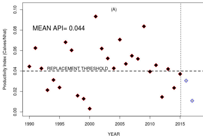
Figure 3. Productivity in the North Atlantic right whale population as characterized by calves detected/ (N_{est}) . The N_{est} values are the model-based estimates of Figure 2(A). Note that the 2016 and 2017 values assume the 2015 estimated abundance.
