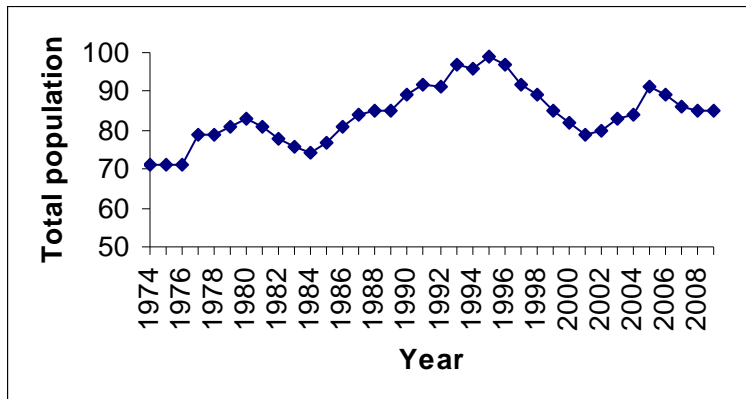
Figure 2. Population of Eastern North Pacific Southern Resident stock of killer whales, 1974-2009. Each year's count includes animals first seen and first missed; a whale is considered first missed the year after it was last seen alive (Ford et al. 2000; Center for Whale Research, unpubl. data).
